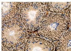
DF7687 at 1/100 staining Mouse testis tissue by IHC-P. The sample was formaldehyde fixed and a heat mediated antigen retrieval step in citrate buffer was performed. The sample was then blocked and incubated with the primary Ab at 4°C overnight. An HRP conjugated anti-Rabbit Ab was used as the secondary Ab.
