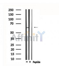
Western blot analysis of extracts from rat brain, using TESK2 Ab.
